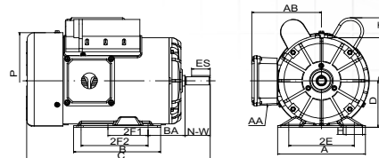
Figure 1 48 thru 140T (Foot Mounting)
